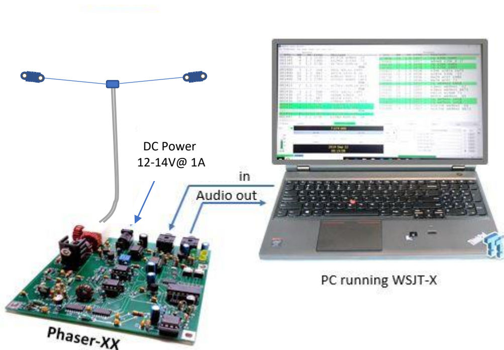
Figure 4: Connecting the Phaser Board to a Computer
