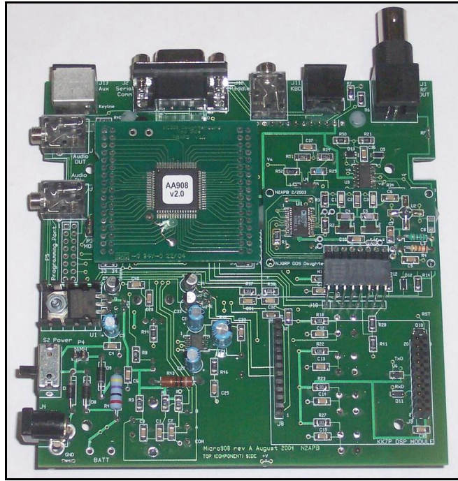
Top/Component Side
